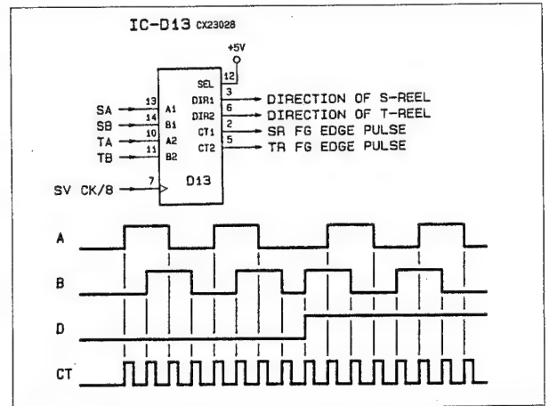
Fig. 4-4-7. Rotation Direction/Rotational Speed Sensing (RS-23 Board)
